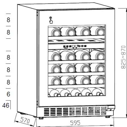
Fig. 4 - Example of the arrangement of 46 standard 750-ml Bordeaux bottles.
