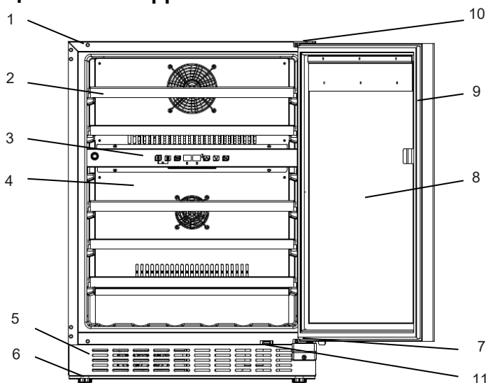
Fig. 2 - Main parts of the appliance.
